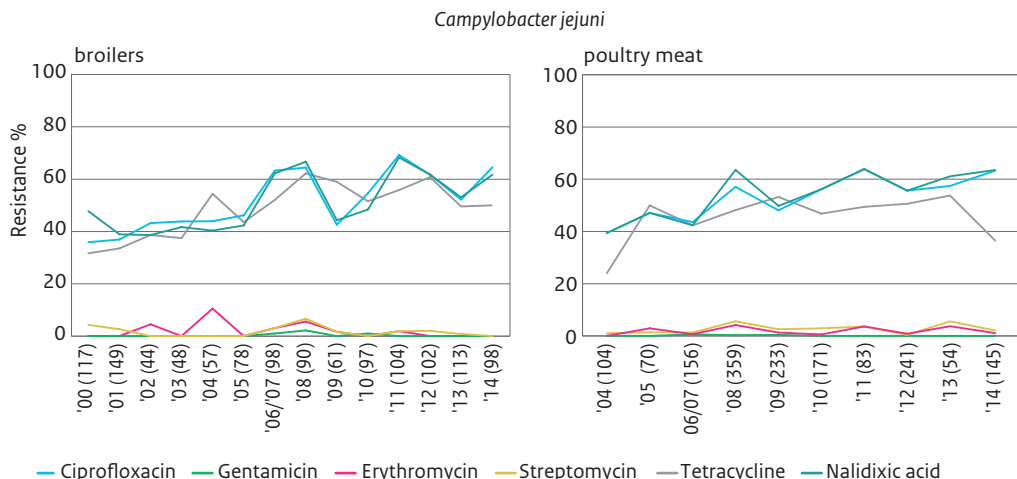
Figure Co1 Trends in resistance (%) of Campylobacter jejuni isolated from broilers and poultry meat in the Netherlands.
